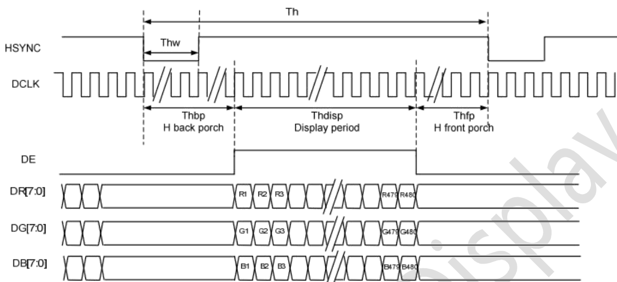
DE Mode Timing Diagram
